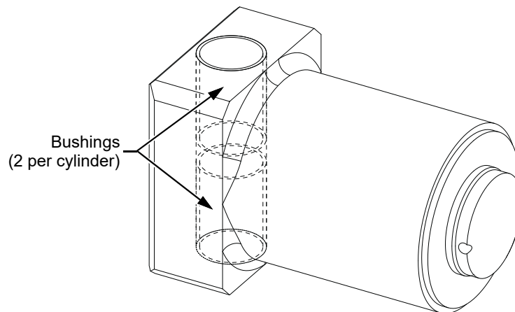
Figure 1: Clamp cylinder bushings
