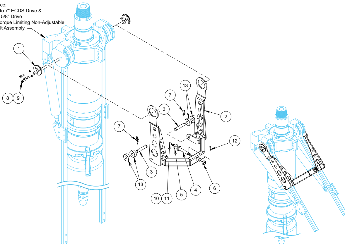
Figure 1: Stabilizer Kit #5104015
