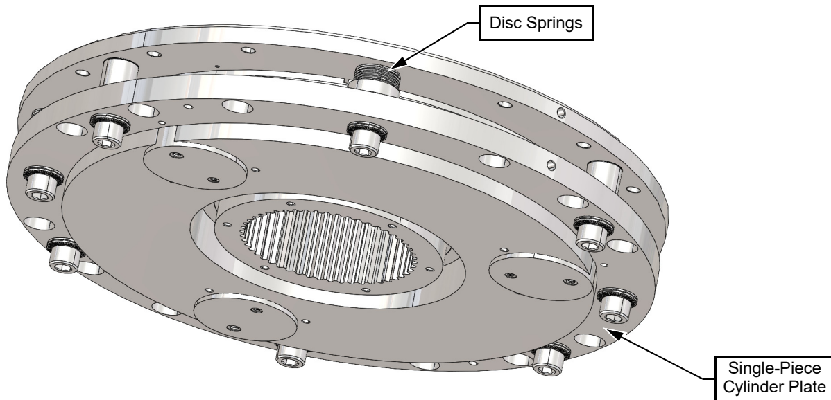
Figure 2: M15601 / New Brake Assembly
