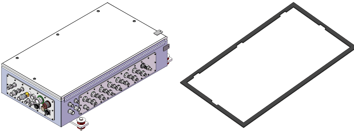
Figure 6: PLC JBox Enclosure DT36220 and Replacement Gasket DT36220-1
