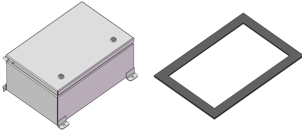
Figure 3: Aux. Motor JBox Enclosure DT24735 and Replacement Gasket DT24735-1
