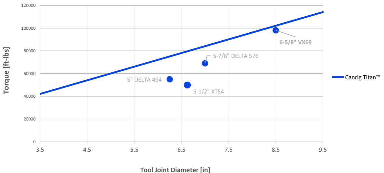
Slip Line Torque vs. Tool Joint Diameter
